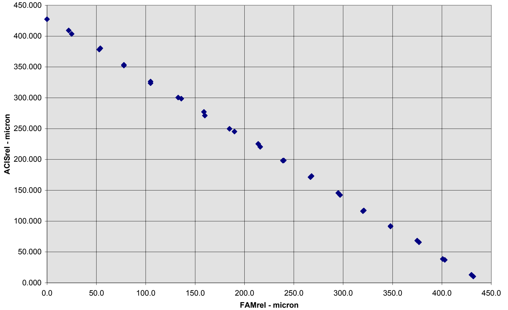
ACISrel v. FAMrel (Horizontal - Sim. Int.) ACIS X = 429.062 - 0.96815 * FAM Y
